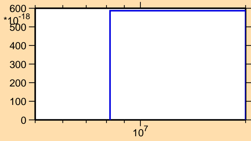
\sigma vs. E for ^{172}\text{Dy}(n,3n\alpha)
