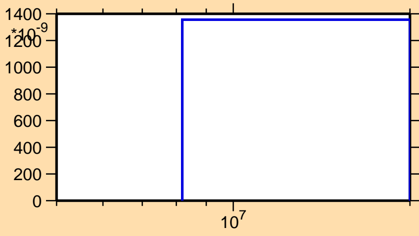
\sigma vs. E for ^{172}\text{Dy}(n,d)
