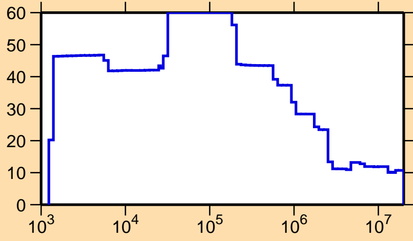
\Delta\sigma/\sigma vs. E for ^{173}\text{Dy}(n,\text{nonel.})
