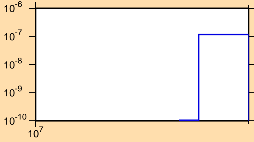
\sigma vs. E for ^{173}\text{Dy}(n,nd)
