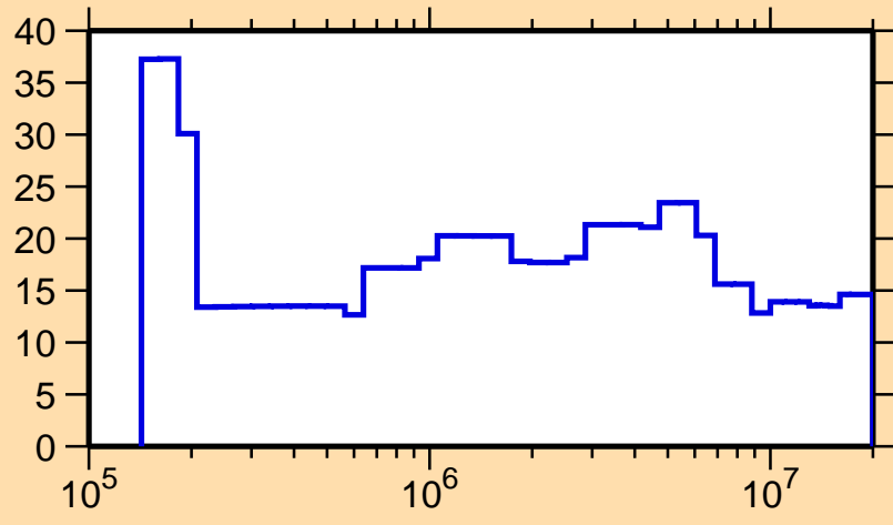
\Delta\sigma/\sigma vs. E for ^{173}\text{Dy}(n,\text{el.})
