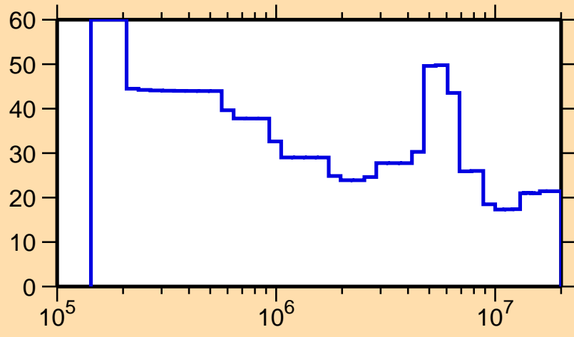
\Delta\sigma/\sigma vs. E for ^{173}\text{Dy}(n,\text{inel.})
