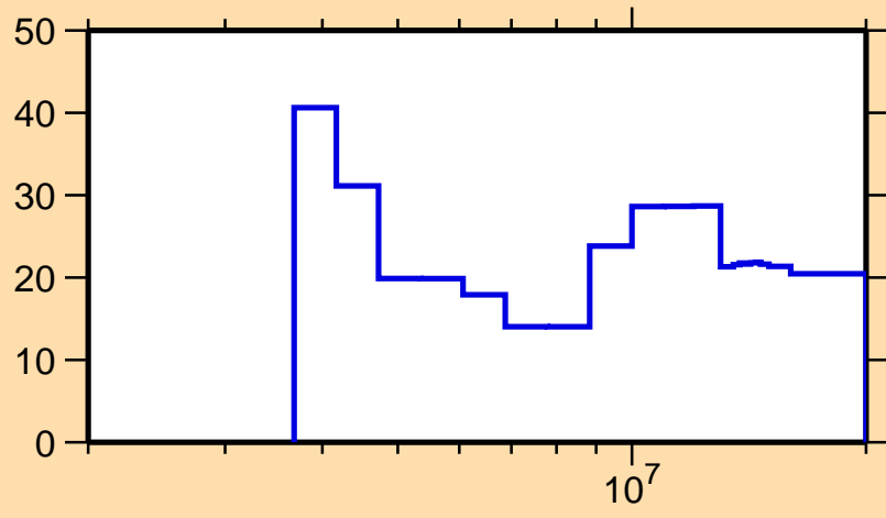
\Delta\sigma/\sigma vs. E for ^{173}\text{Dy}(n,2n)
