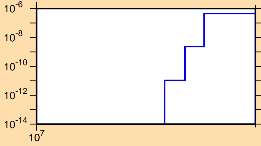
\sigma vs. E for ^{173}\text{Dy}(n,nt)
