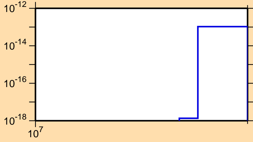
\sigma vs. E for ^{173}\text{Dy}(n,3n\alpha)
