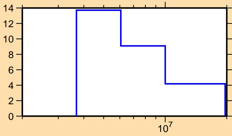
\Delta\sigma/\sigma vs. E for ^{173}\text{Dy}(n,\text{tot.})
