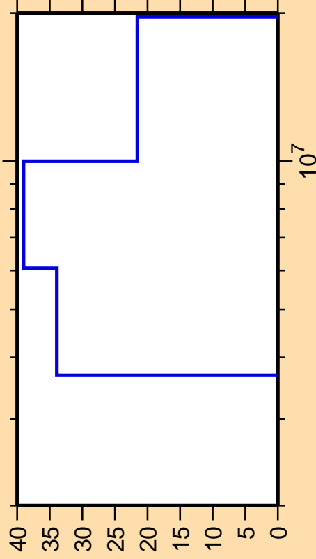
\Delta\sigma/\sigma vs. E for ^{173}\text{Dy}(n,n\text{cont.})
