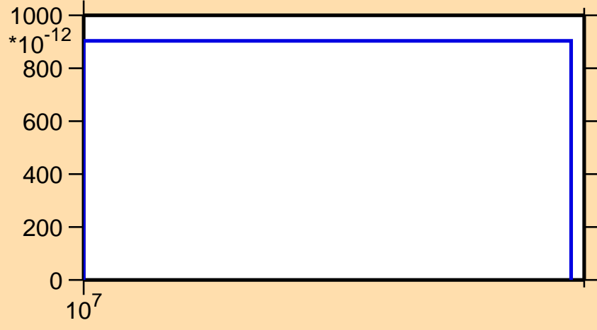
\sigma vs. E for ^{173}\text{Dy}(n,nd)
