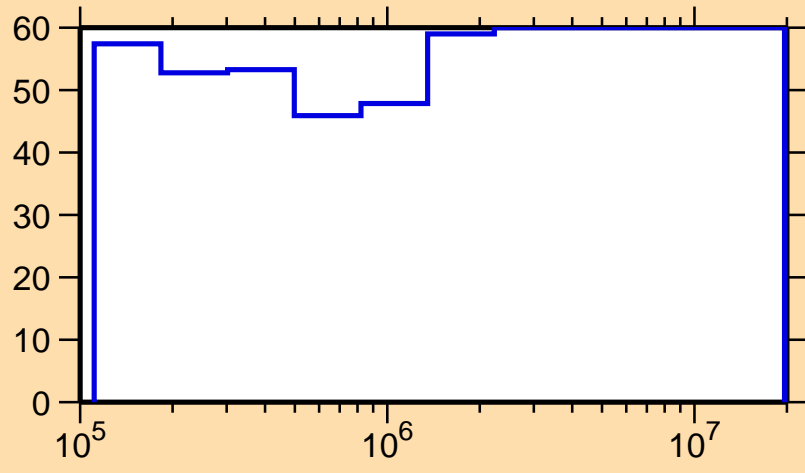
\Delta\sigma/\sigma vs. E for ^{173}\text{Dy}(n,n_1)
