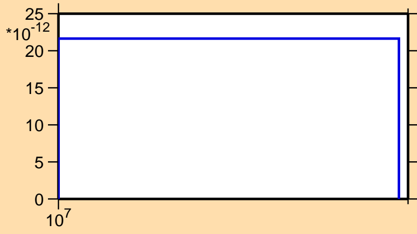
\sigma vs. E for ^{173}\text{Dy}(n,2np)
