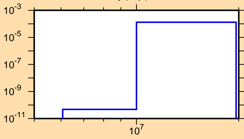
\sigma vs. E for ^{173}\text{Dy}(n,p)
