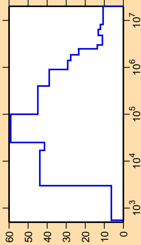
\Delta\sigma/\sigma vs. E for ^{173}\text{Dy}(n,\text{nonel.})
