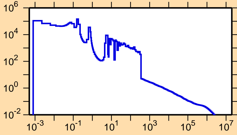
\sigma vs. E for ^{146}\text{Er}(n,\gamma)
