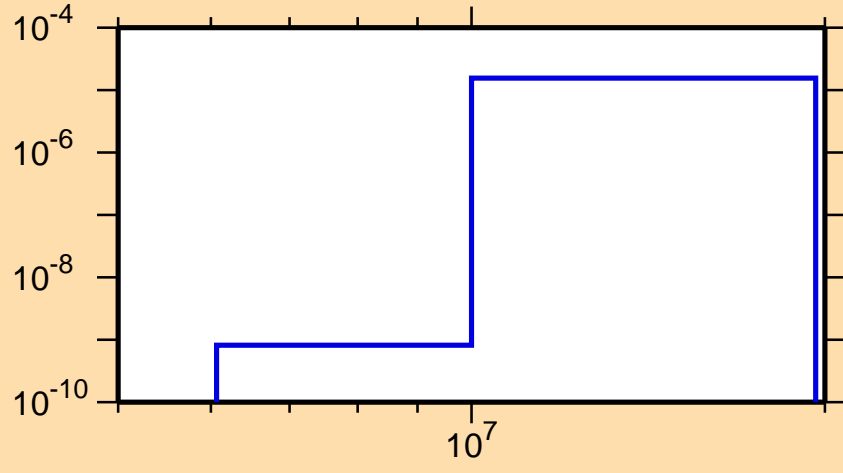
\sigma vs. E for ^{146}\text{Er}(\text{mt } 45)
