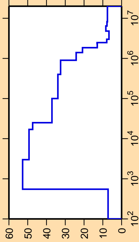
\Delta\sigma/\sigma vs. E for ^{146}\text{Er}(n,\text{nonel.})
