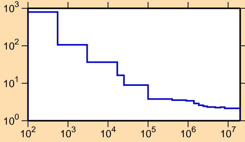
\sigma vs. E for ^{146}\text{Er}(n,\text{nonel.})
