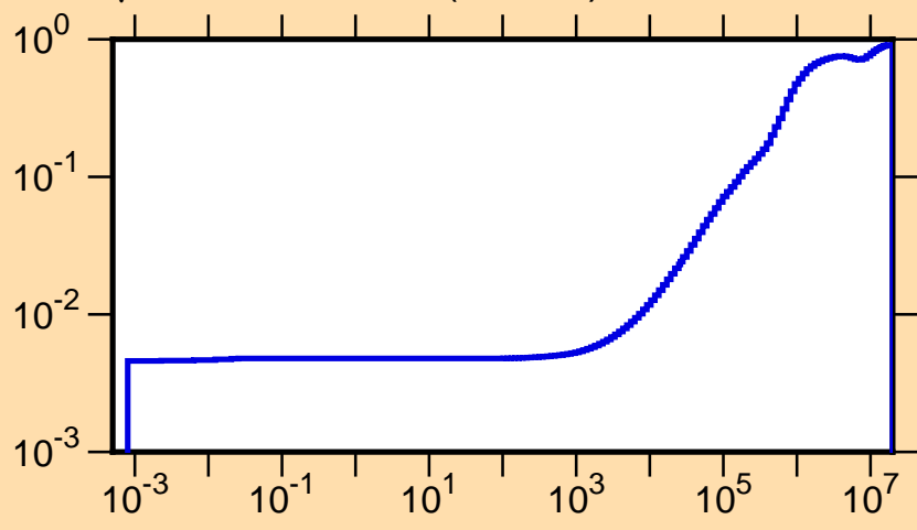
\mu vs. E for ^{147}\text{Er}(\text{mt251})
