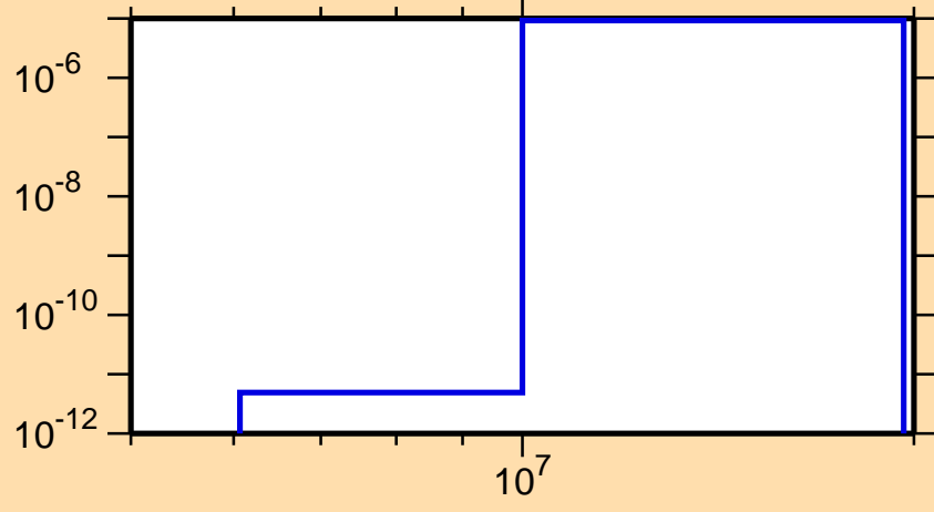
\sigma vs. E for ^{147}\text{Er} (mt 45)
