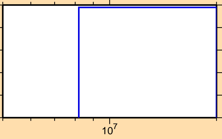
\sigma vs. E for ^{147}\text{Er}(\text{mt } 34)
