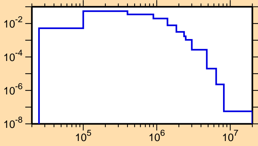
\sigma vs. E for ^{147}\text{Er}(n,n_1)
