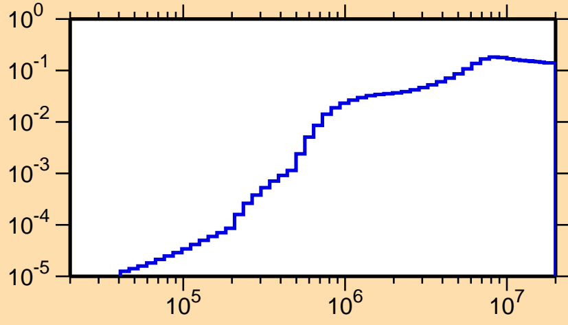
\sigma vs. E for ^{147}\text{Er}(n,\text{inel.})
