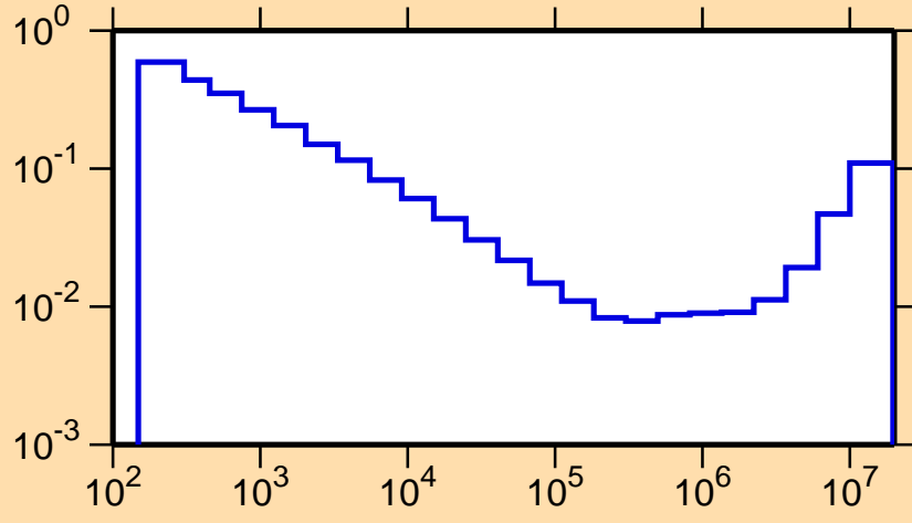
\sigma vs. E for ^{147}\text{Er}(n,\alpha)
