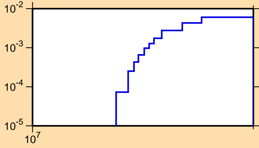
\sigma vs. E for ^{148}\text{Er}(n,2n)
