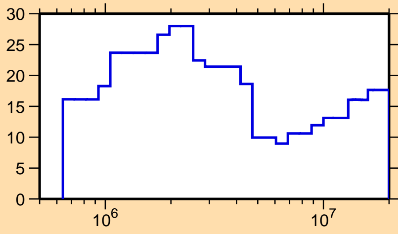
\Delta\sigma/\sigma vs. E for ^{148}\text{Er}(n,\text{tot.})
