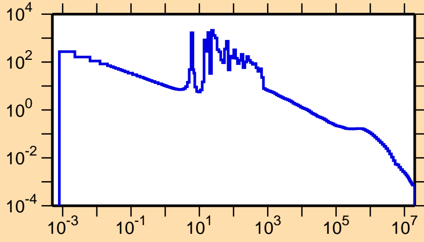
\sigma vs. E for ^{148}\text{Er}(n,\gamma)
