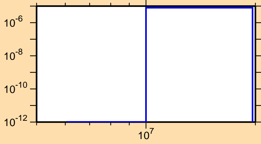
\sigma vs. E for ^{148}\text{Er}(\text{mt } 45)
