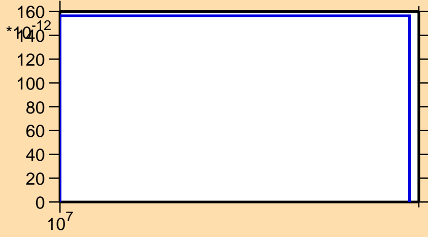
\sigma vs. E for ^{149}\text{Er} (mt 34)
