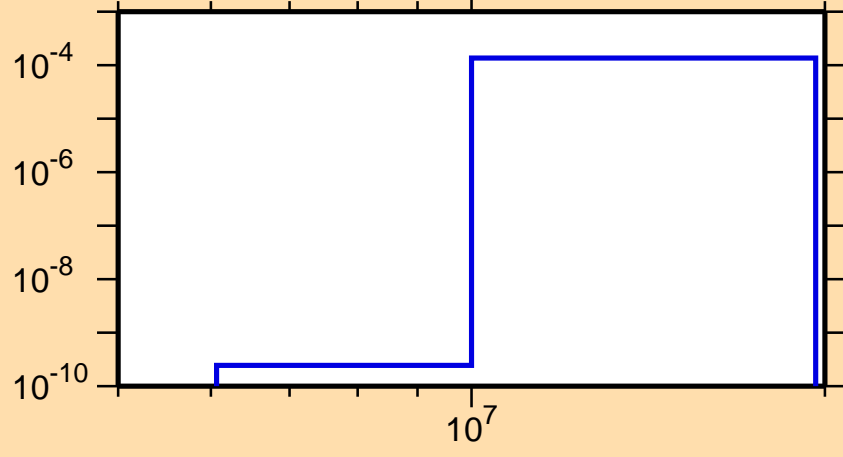
\sigma vs. E for ^{149}\text{Er}(n,\text{pd})
