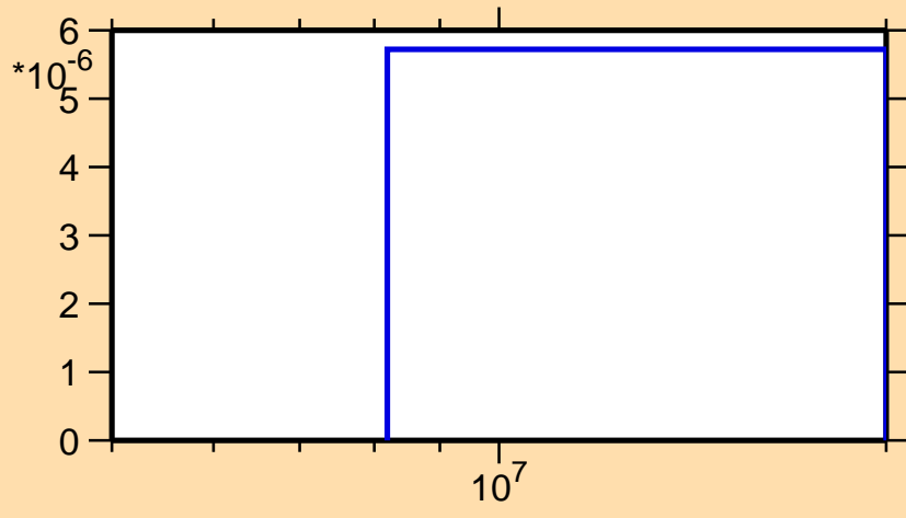
\sigma vs. E for ^{149}\text{Er}(n,2np)
