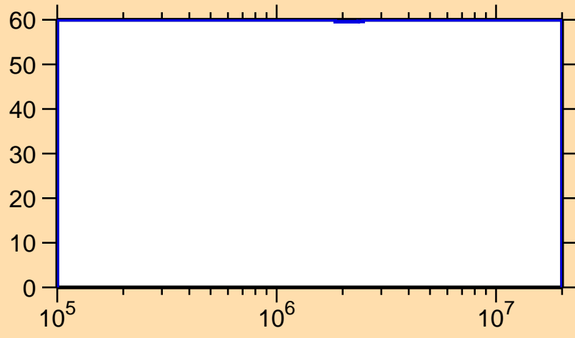
\Delta\sigma/\sigma vs. E for ^{149}\text{Er}(n,n_1)
