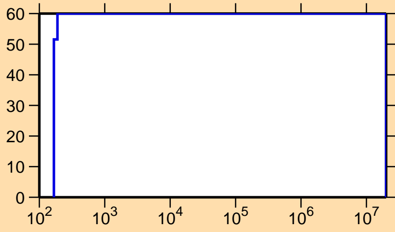
\Delta\sigma/\sigma vs. E for ^{149}\text{Er}(n,\gamma)
