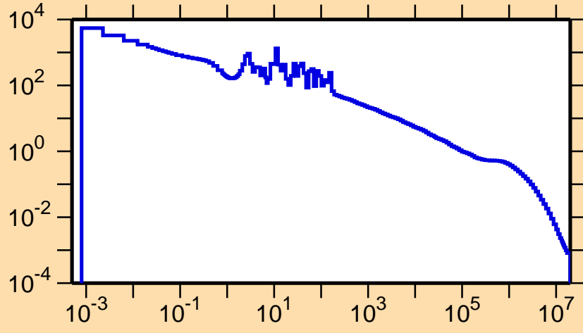
\sigma vs. E for ^{149}\text{Er}(n,\gamma)
