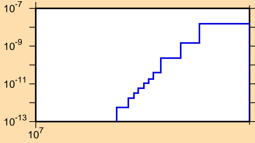
\sigma vs. E for ^{149}\text{Er}(\text{mt } 34)
