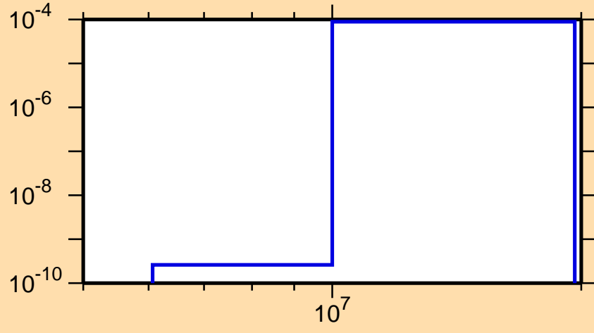
\sigma vs. E for ^{149}\text{Er}(n,\text{pd})
