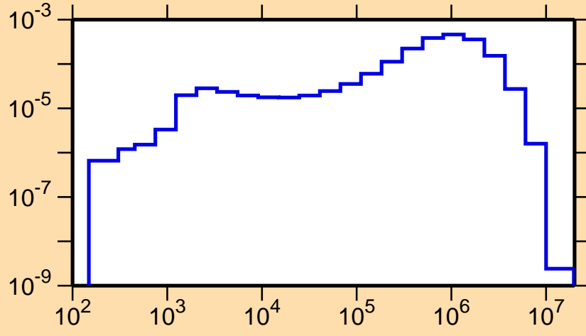
\sigma vs. E for ^{149}\text{Er}(n,n_1)
