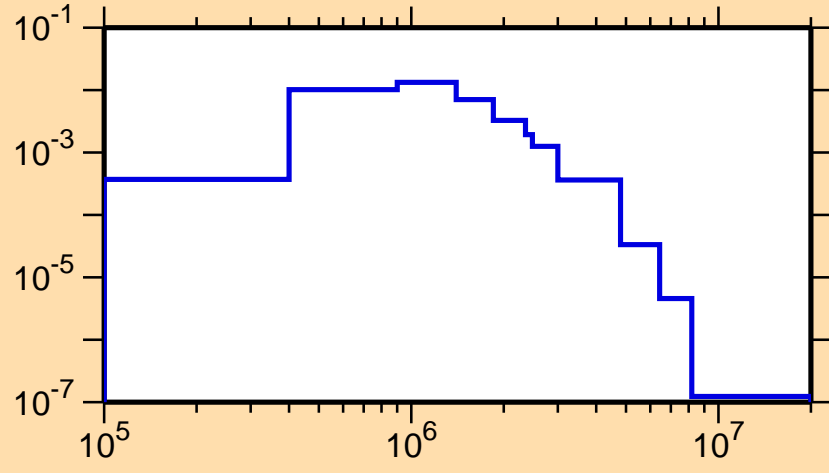
\sigma vs. E for ^{149}\text{Er}(n,n_4)
