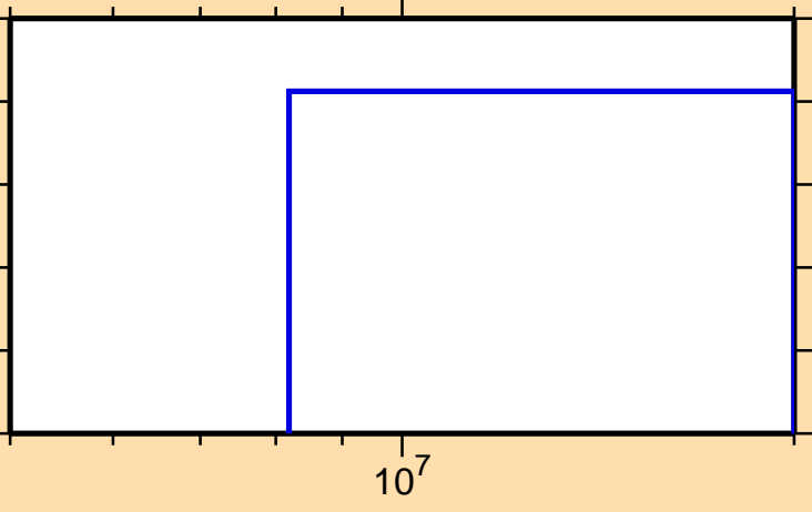
\sigma vs. E for ^{149}\text{Er}(n,2n\alpha)
