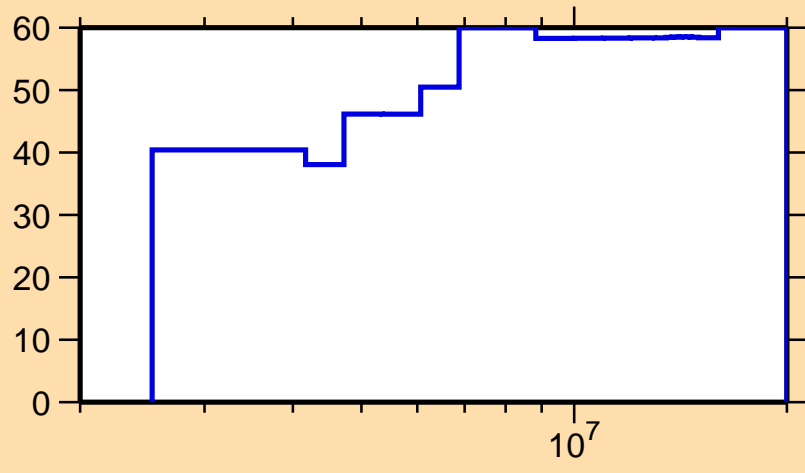
\Delta\sigma/\sigma vs. E for ^{151}\text{Er}(n,n\text{cont.})
