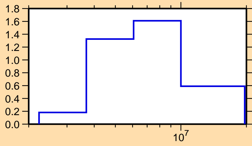
\sigma vs. E for ^{151}\text{Er}(n,n\text{cont.})
