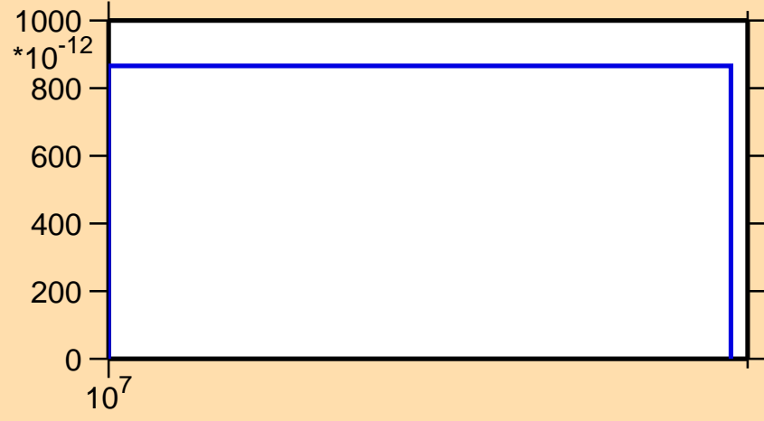
\sigma vs. E for ^{151}\text{Er} (mt 34)
