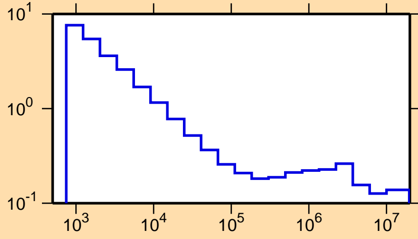
\sigma vs. E for ^{151}\text{Er}(n,\alpha)
