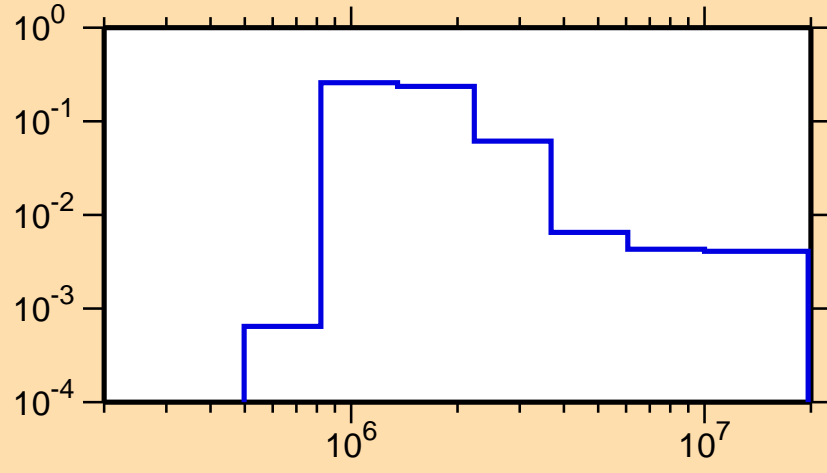
\sigma vs. E for ^{151}\text{Er}(n,n_1)
