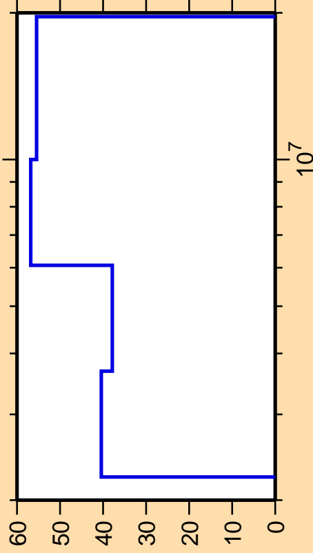
\Delta\sigma/\sigma vs. E for ^{151}\text{Er}(n,n\text{cont.})
