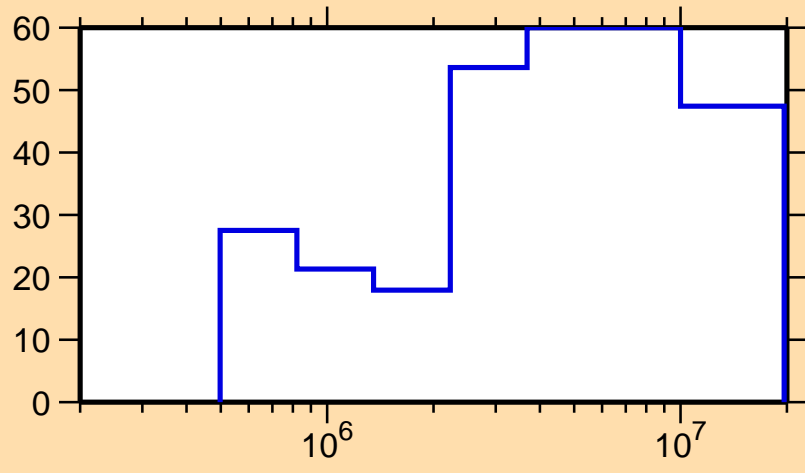
\Delta\sigma/\sigma vs. E for ^{151}\text{Er}(n,\text{el.})
