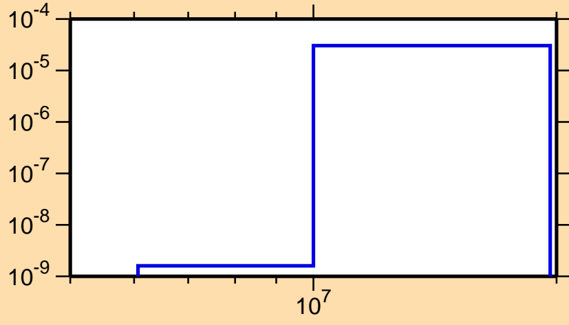
\sigma vs. E for ^{151}\text{Er}(\text{mt } 45)
