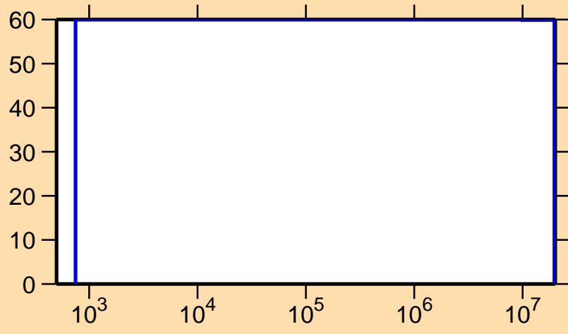
\Delta\sigma/\sigma vs. E for ^{151}\text{Er}(n,\gamma)
