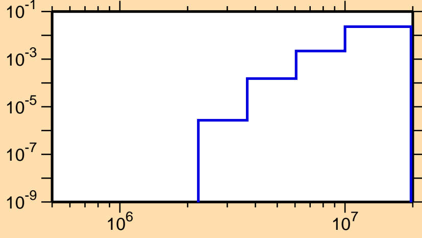
\sigma vs. E for ^{151}\text{Er}(n,n\alpha)
