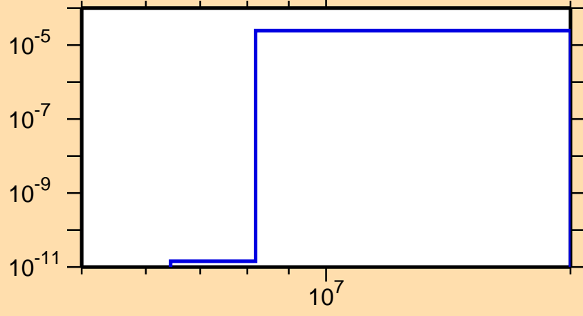
\sigma vs. E for ^{151}\text{Er} (mt 45)
