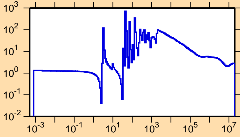
\sigma vs. E for ^{152}\text{Er}(n,\text{el.})
