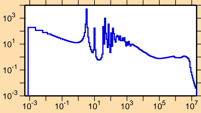
\sigma vs. E for ^{152}\text{Er}(n,\gamma)
