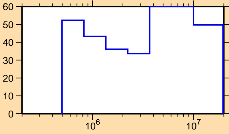
\Delta\sigma/\sigma vs. E for ^{152}\text{Er}(n,n_1)
