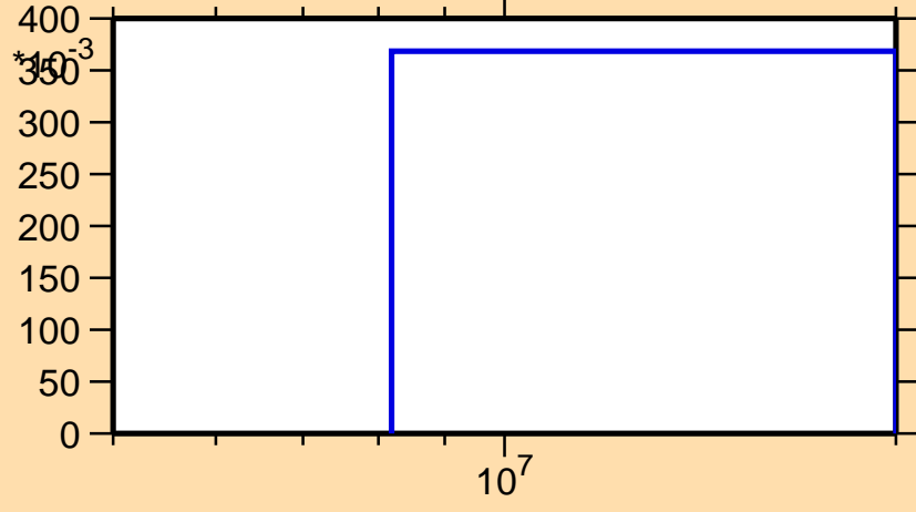
\sigma vs. E for ^{152}\text{Er}(n,2n)
