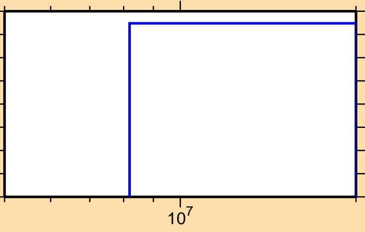
\sigma vs. E for ^{152}\text{Er}(n,\text{nd})
