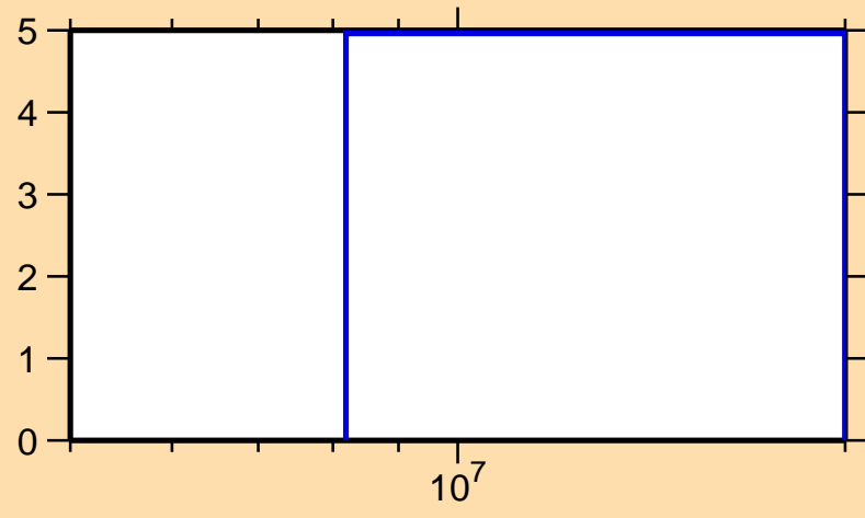
\Delta\sigma/\sigma vs. E for ^{152}\text{Er}(n,\text{nonel.})
