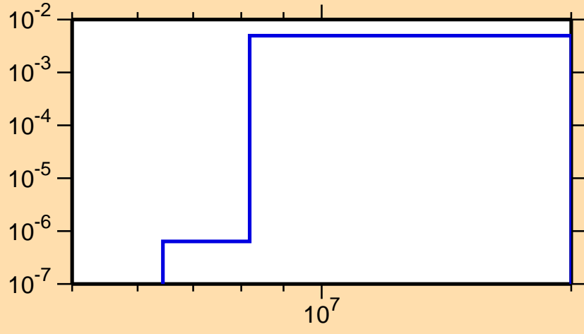
\sigma vs. E for ^{152}\text{Er}(\text{mt } 45)
