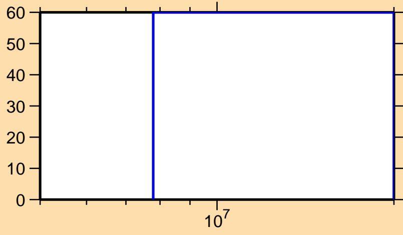
\Delta\sigma/\sigma vs. E for ^{153}\text{Er}(n,2n)
