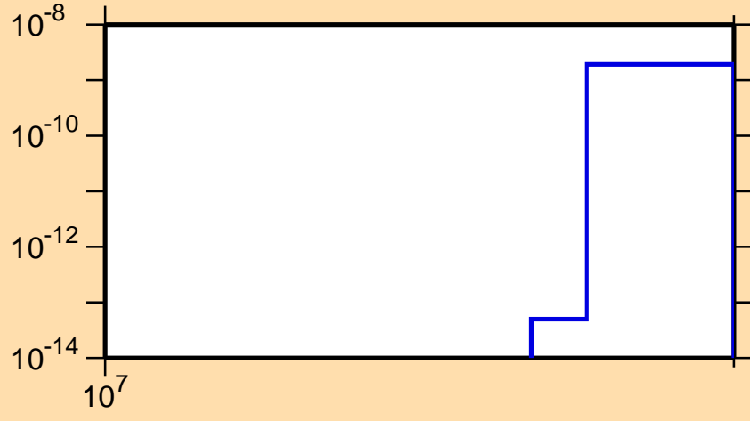
\sigma vs. E for ^{153}\text{Er}(n,nt)
