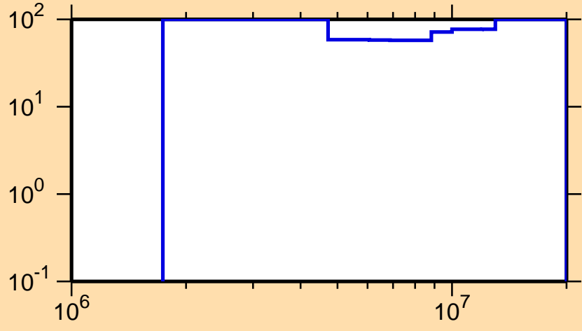
\Delta\sigma/\sigma vs. E for ^{153}\text{Er}(n,n\text{cont.})
