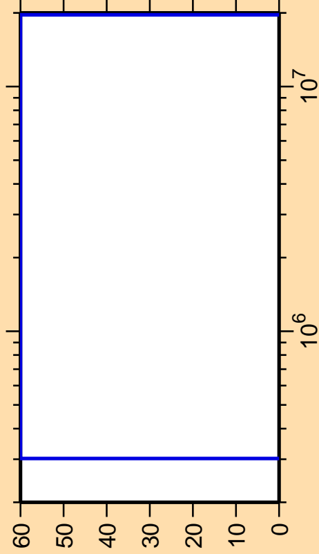
\Delta\sigma/\sigma vs. E for ^{153}\text{Er}(n,n_2)
