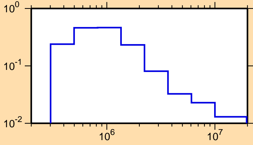
\sigma vs. E for ^{153}\text{Er}(n,n_2)
