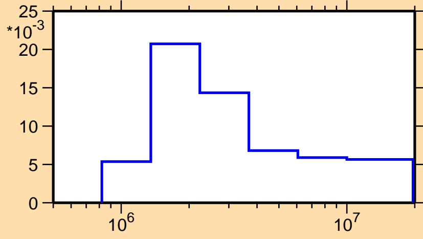
\sigma vs. E for ^{153}\text{Er}(n,n_4)
