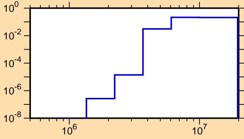
\sigma vs. E for ^{153}\text{Er}(n,n\alpha)
