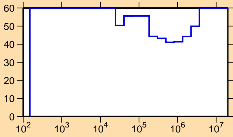
\Delta\sigma/\sigma vs. E for ^{153}\text{Er}(n,\gamma)
