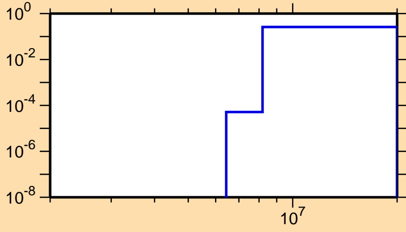
\sigma vs. E for ^{153}\text{Er}(n,np)
