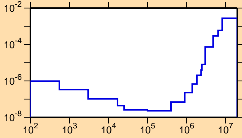
\sigma vs. E for ^{153}\text{Er}(n,p\alpha)
