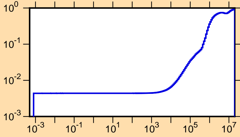
\mu vs. E for ^{154}\text{Er}(\text{mt251})
