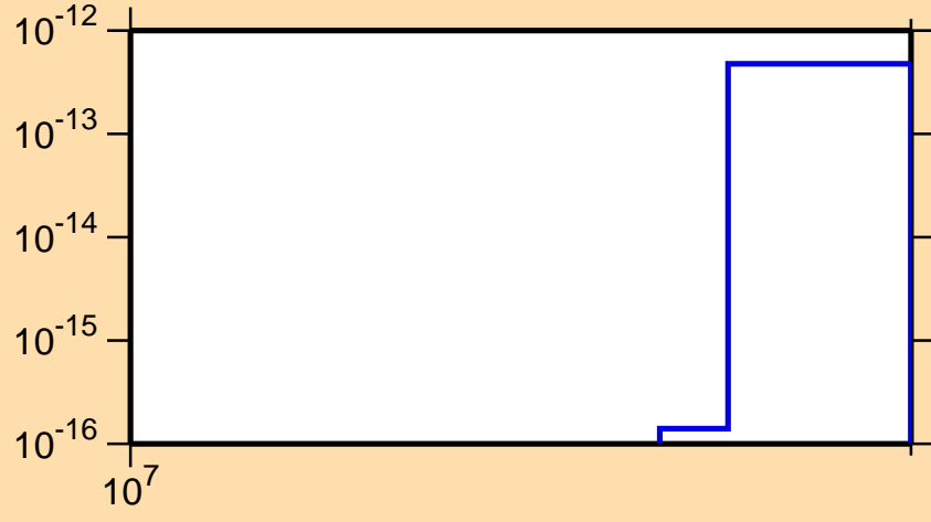
\sigma vs. E for ^{154}\text{Er}(n,3n\alpha)
