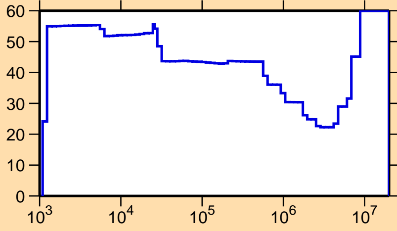
\Delta\sigma/\sigma vs. E for ^{154}\text{Er}(n,\gamma)
