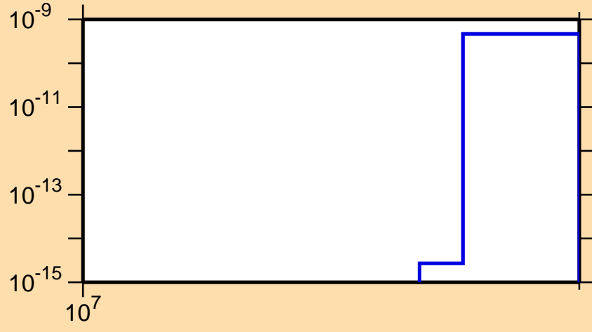
\sigma vs. E for ^{154}\text{Er}(n,nt)
