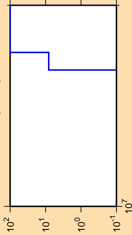
\Delta\sigma/\sigma vs. E for ^{154}\text{Er} (mt 34)
