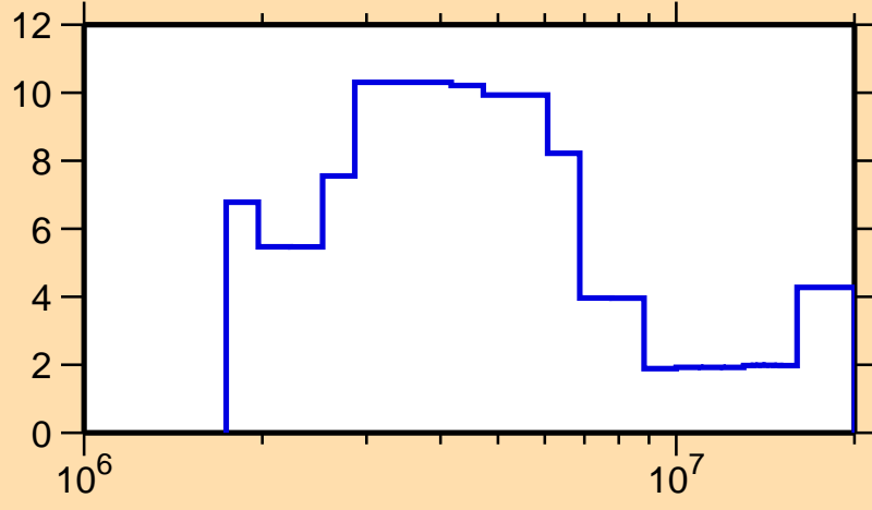
\Delta\sigma/\sigma vs. E for ^{154}\text{Er}(n,\text{tot.})
