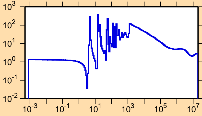
\sigma vs. E for ^{154}\text{Er}(n,\text{el.})
