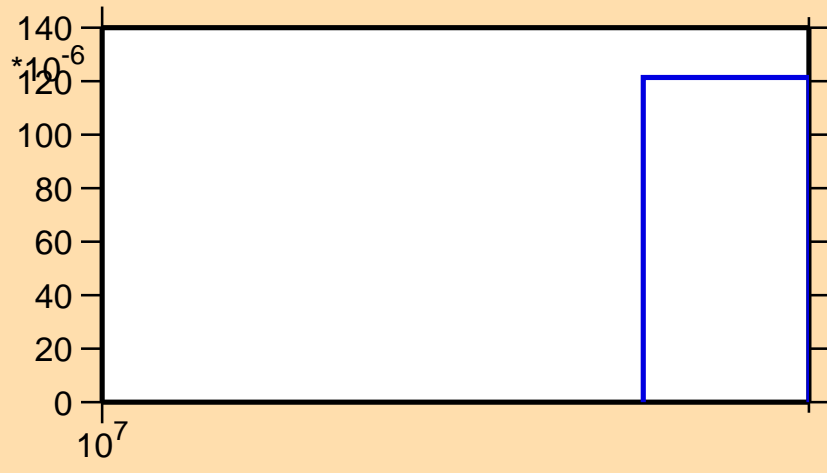
\sigma vs. E for ^{154}\text{Er}(n,3n)
