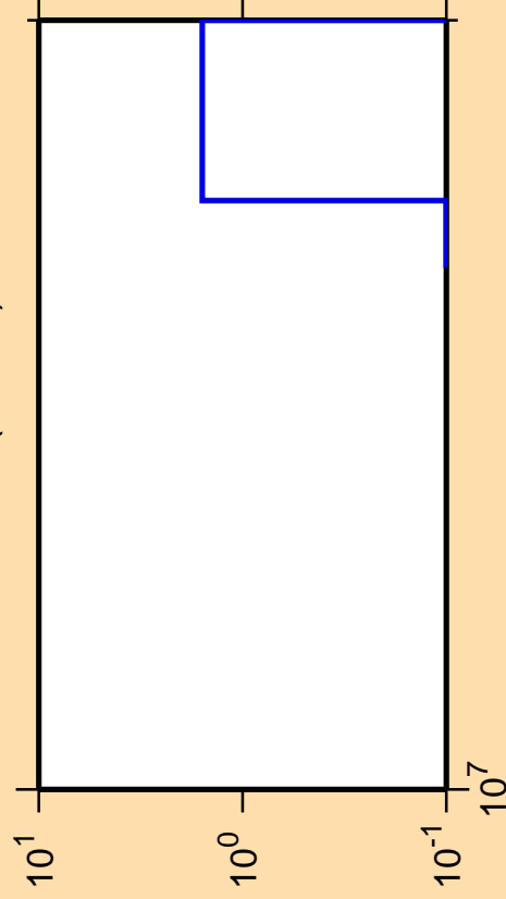
\Delta\sigma/\sigma vs. E for ^{154}\text{Er}(n,3n\alpha)
