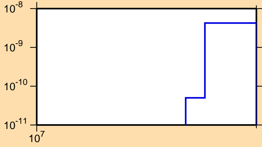
\sigma vs. E for ^{154}\text{Er}(n,\text{pt})
