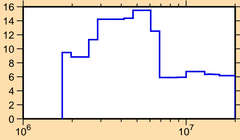
\Delta\sigma/\sigma vs. E for ^{154}\text{Er}(n, \text{el.})
