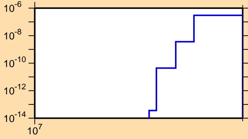
\sigma vs. E for ^{154}\text{Er}(n,\text{nd})
