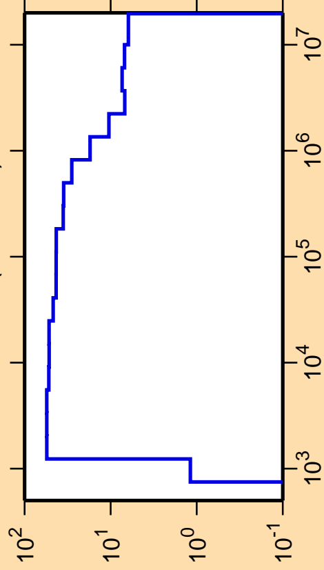
\Delta\sigma/\sigma vs. E for ^{154}\text{Er}(n,\text{nonel.})
