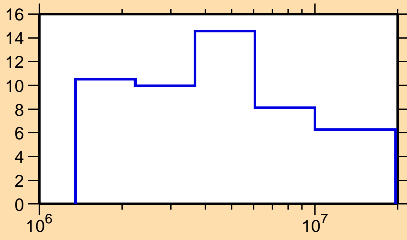
\Delta\sigma/\sigma vs. E for ^{154}\text{Er}(n, el.)
