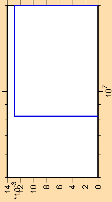
\Delta\sigma/\sigma vs. E for ^{154}\text{Er}(n,3n\alpha)
