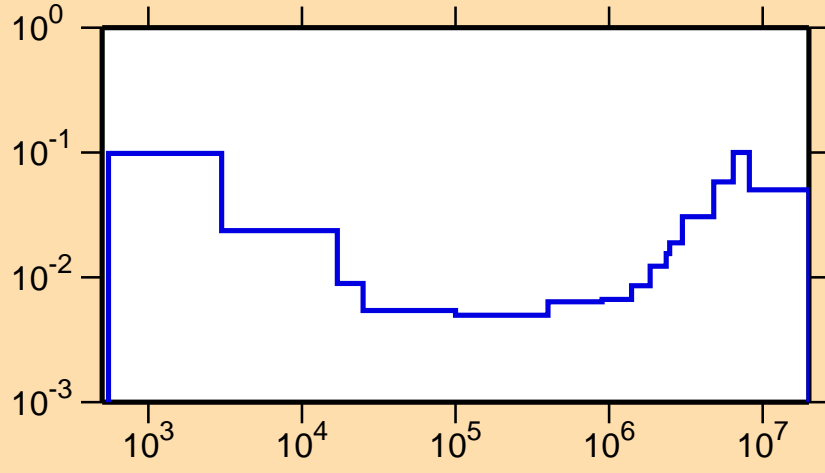
\sigma vs. E for ^{154}\text{Er}(n,\alpha)
