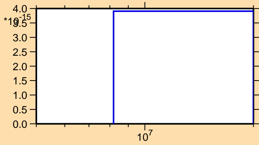
\sigma vs. E for ^{154}\text{Er}(n,3n\alpha)
