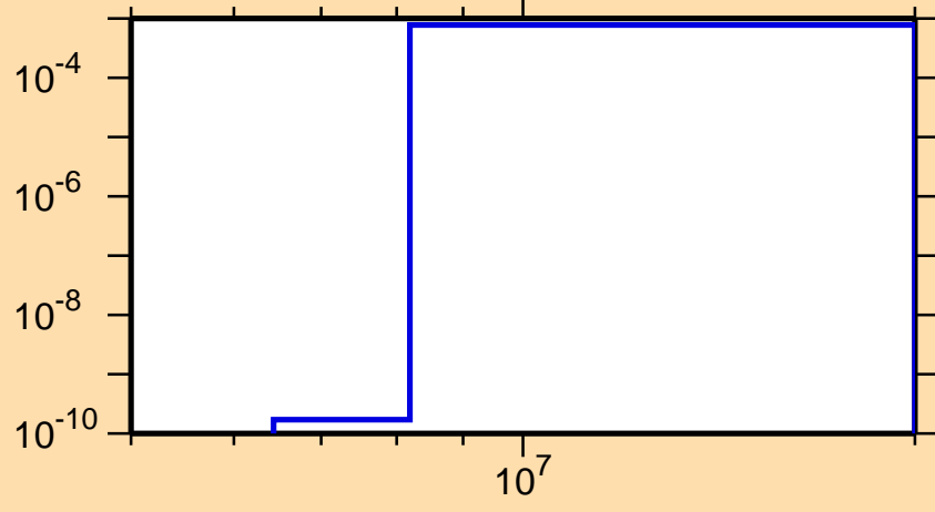
\sigma vs. E for ^{154}\text{Er} (mt 45)
