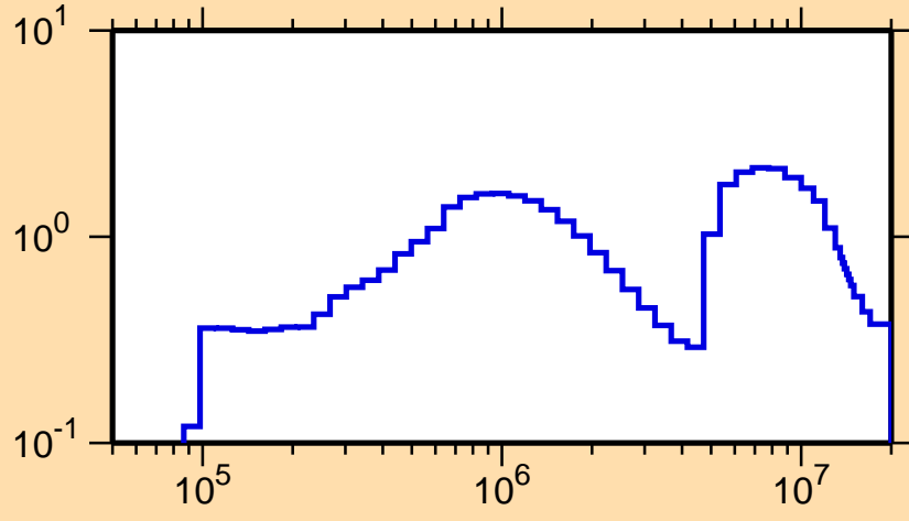
\sigma vs. E for ^{155}\text{Er}(n,\text{inel.})
