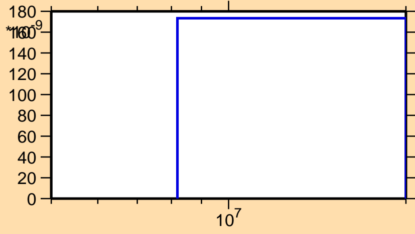
\sigma vs. E for ^{155}\text{Er} (mt 45)
