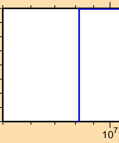
\sigma vs. E for ^{155}\text{Er}(n,2n\alpha)
