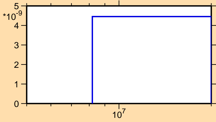
\sigma vs. E for ^{155}\text{Er}(\text{mt117})
