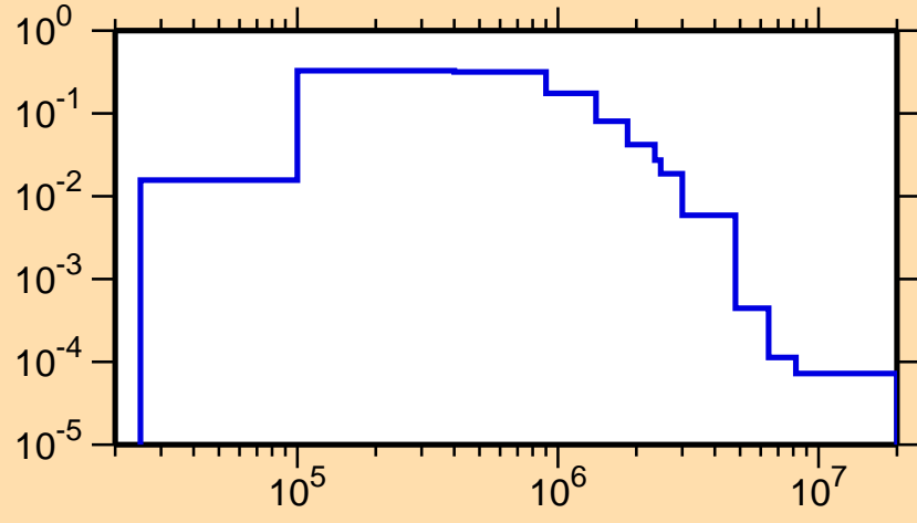
\sigma vs. E for ^{155}\text{Er}(n,n_1)
