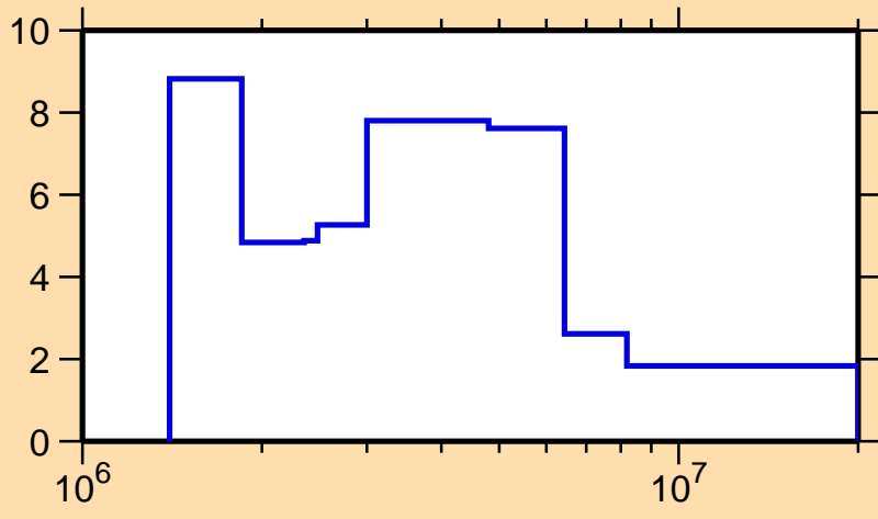
\Delta\sigma/\sigma vs. E for ^{155}\text{Er}(n,\text{tot.})
