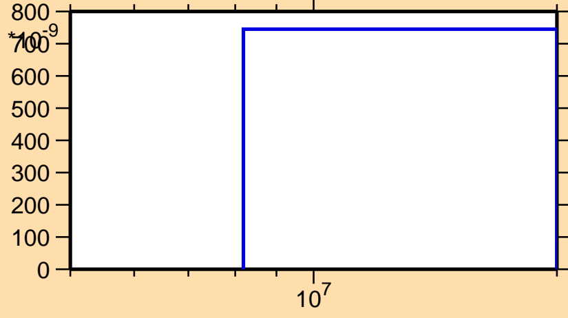
\sigma vs. E for ^{155}\text{Er}(n,\text{He}3)
