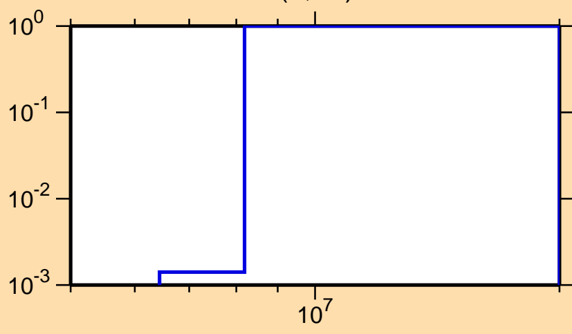
\sigma vs. E for ^{155}\text{Er}(n,2n)
