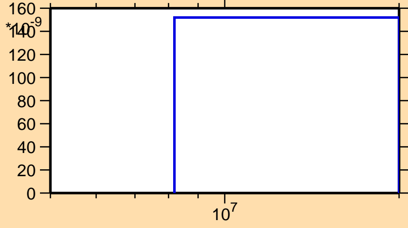
\sigma vs. E for ^{155}\text{Er}(n,\text{nd})
