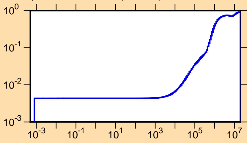
\mu vs. E for ^{156}\text{Er}(\text{mt251})
