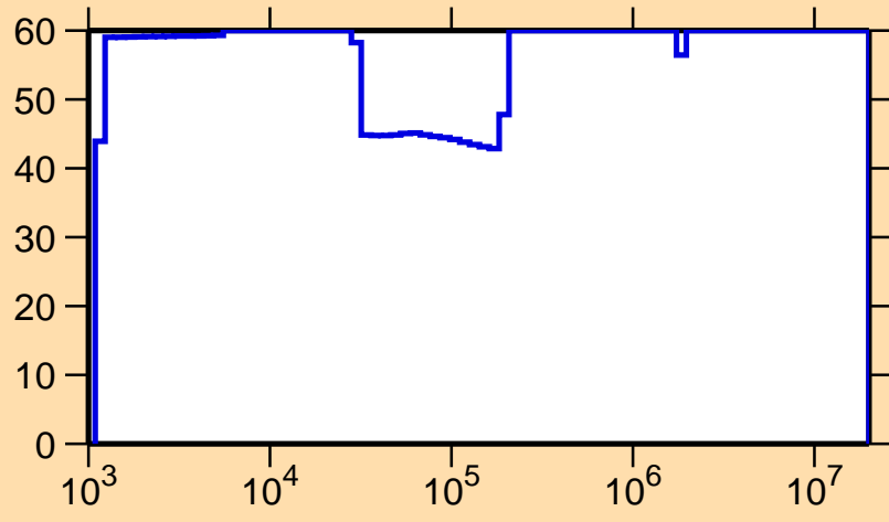
\Delta\sigma/\sigma vs. E for ^{156}\text{Er}(n,\gamma)
