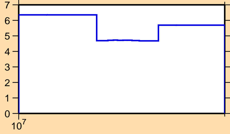
\Delta\sigma/\sigma vs. E for ^{156}\text{Er}(n,\text{tot.})
