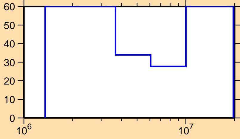
\Delta\sigma/\sigma vs. E for ^{156}\text{Er}(n,n\text{cont.})
