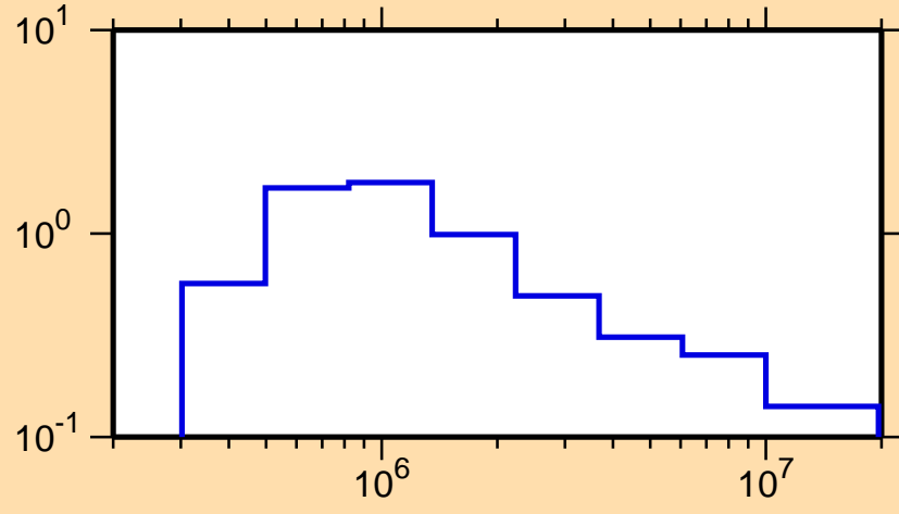
\sigma vs. E for ^{156}\text{Er}(n,n_1)
