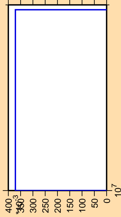
\Delta\sigma/\sigma vs. E for ^{156}\text{Er}(n,\text{pt})
