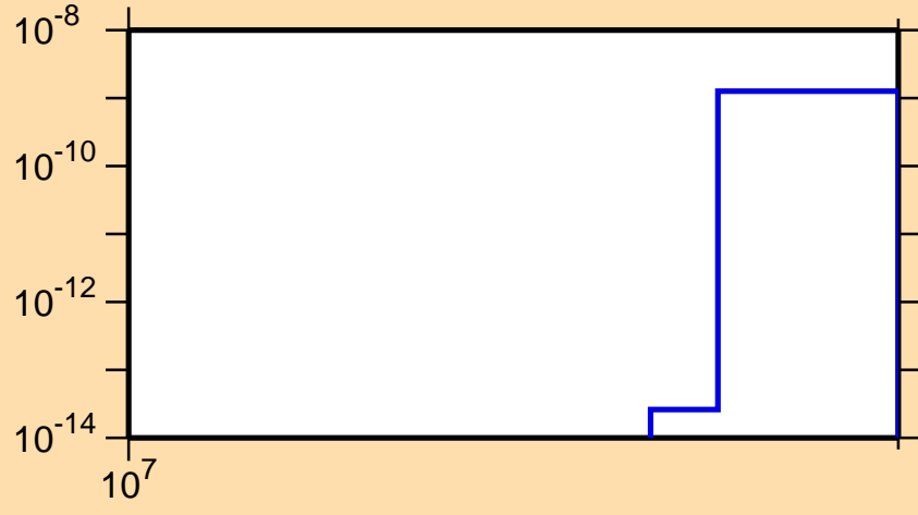
\sigma vs. E for ^{157}\text{Er}(n,nt)
