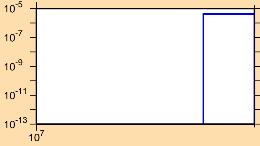
\sigma vs. E for ^{157}\text{Er}(n,3n\alpha)
