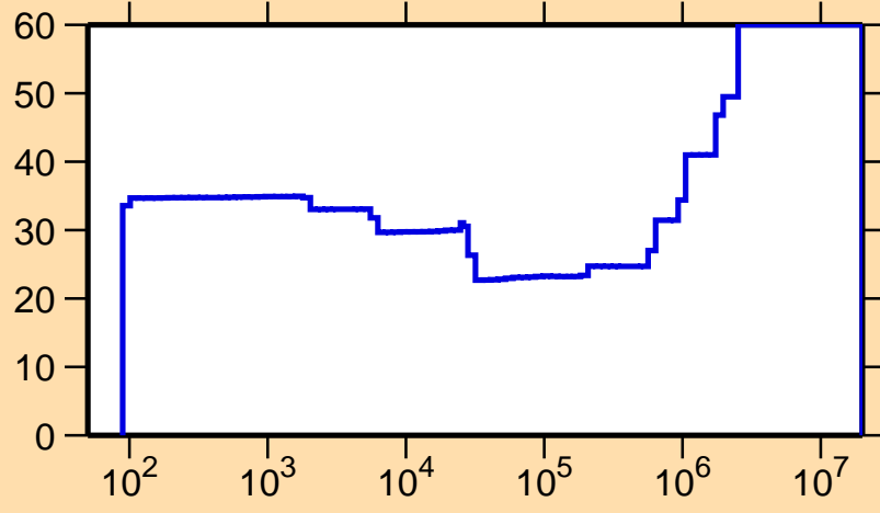
\Delta\sigma/\sigma vs. E for ^{157}\text{Er}(n,\gamma)
