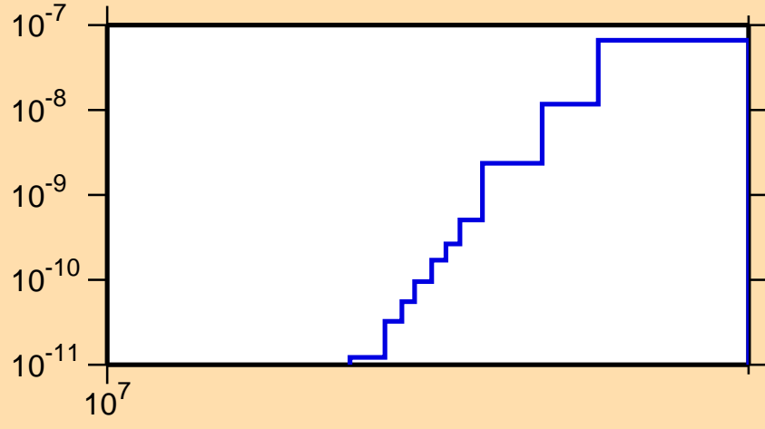
\sigma vs. E for ^{157}\text{Er}(\text{mt } 45)
