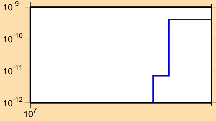
\sigma vs. E for ^{157}\text{Er} (mt 34)
