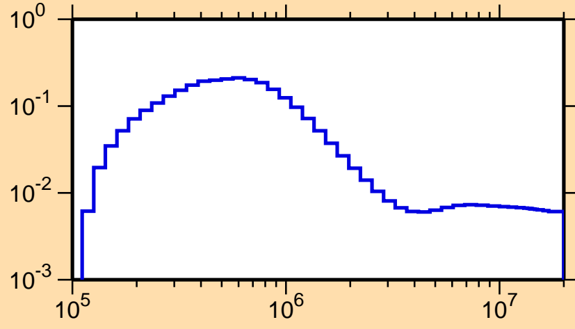
\sigma vs. E for ^{157}\text{Er}(n,n_3)
