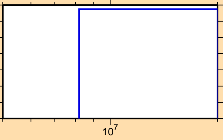
\sigma vs. E for ^{157}\text{Er}(n,3n\alpha)
