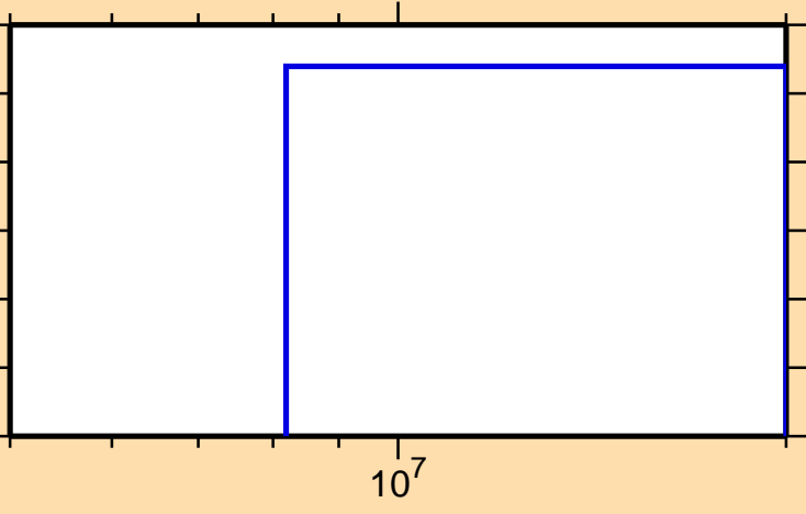
\sigma vs. E for ^{157}\text{Er}(n,3n)
