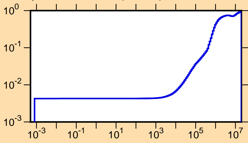
\mu vs. E for ^{158}\text{Er}(\text{mt251})
