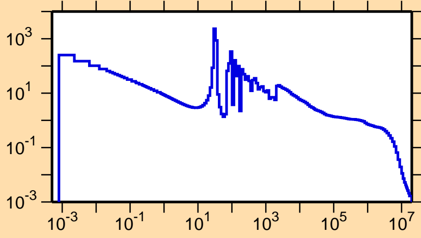
\sigma vs. E for ^{158}\text{Er}(n,\gamma)
