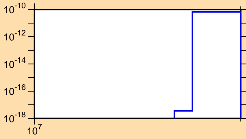
\sigma vs. E for ^{158}\text{Er}(n,3n\alpha)
