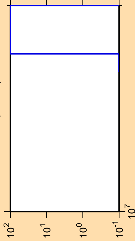
\Delta\sigma/\sigma vs. E for ^{158}\text{Er}(n,3n\alpha)
