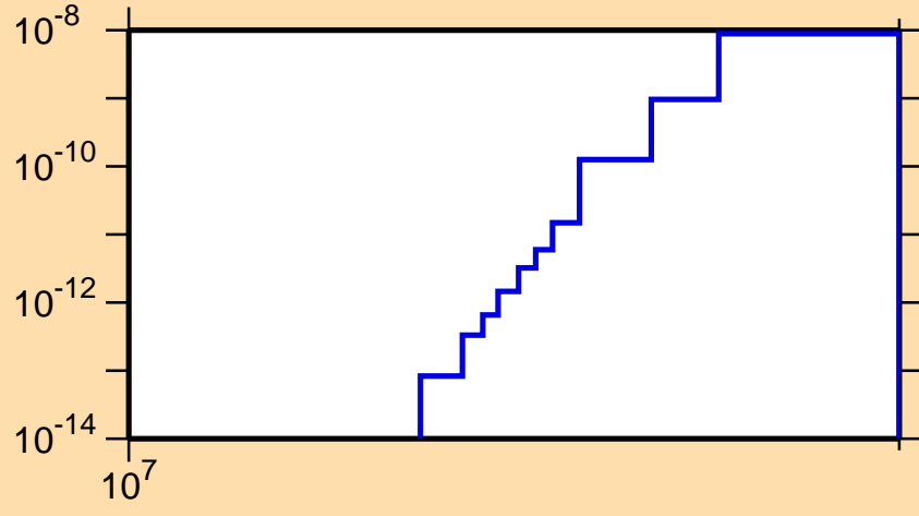
\sigma vs. E for ^{158}\text{Er}(\text{mt } 45)
