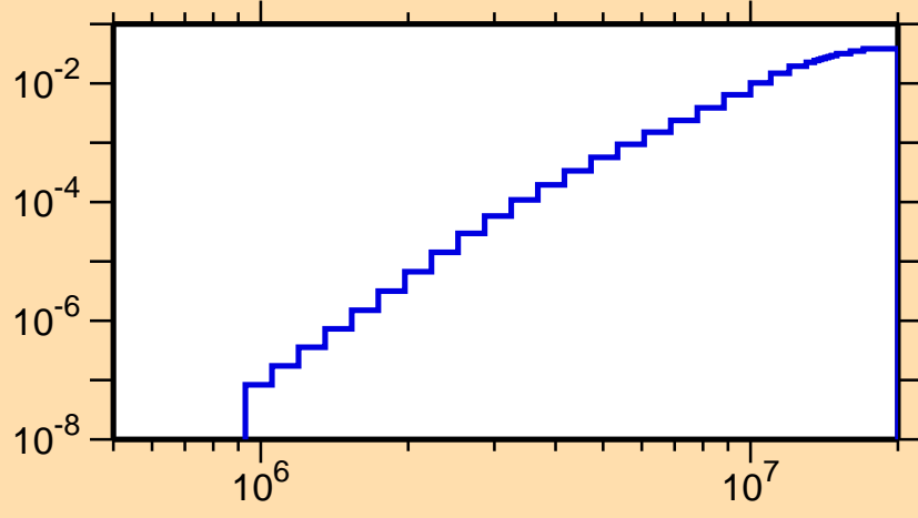
\sigma vs. E for ^{158}\text{Er}(n,p)
