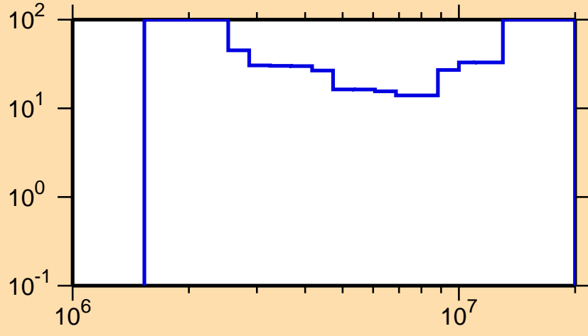
\Delta\sigma/\sigma vs. E for ^{158}\text{Er}(n,n\text{cont.})
