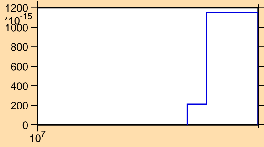
\sigma vs. E for ^{159}\text{Er}(n,3n\alpha)
