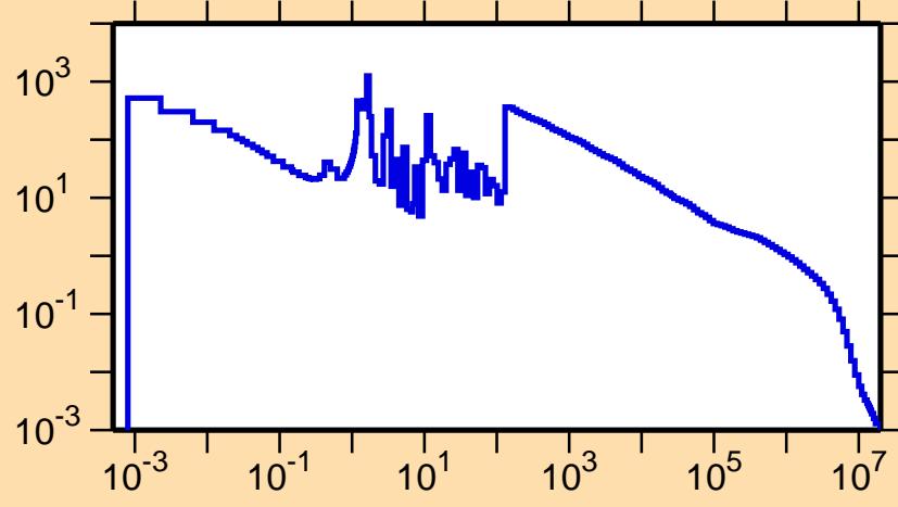
\sigma vs. E for ^{159}\text{Er}(n,\gamma)
