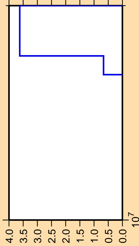
\Delta\sigma/\sigma vs. E for ^{159}\text{Er}(n,3n\alpha)
