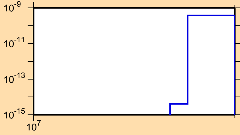
\sigma vs. E for ^{159}\text{Er}(n,nt)
