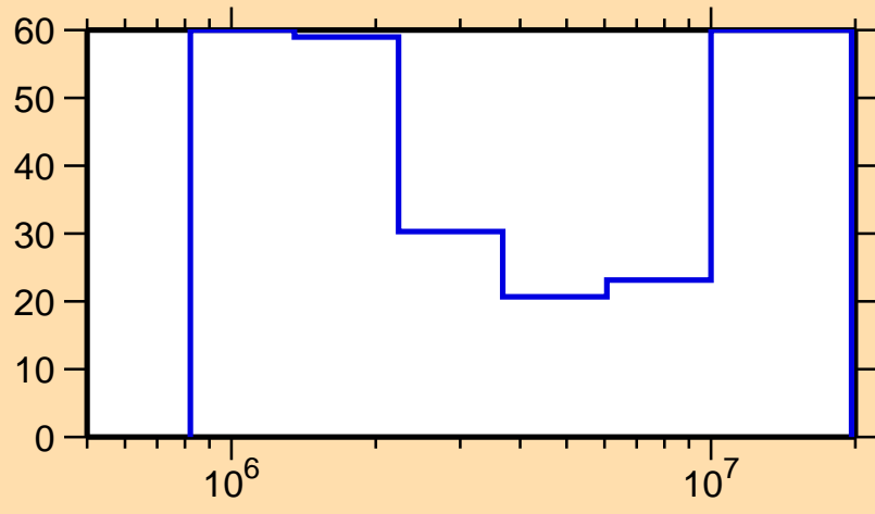
\Delta\sigma/\sigma vs. E for ^{159}\text{Er}(n,n\text{cont.})
