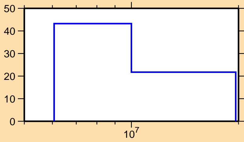
\Delta\sigma/\sigma vs. E for ^{159}\text{Er}(n,2n)
