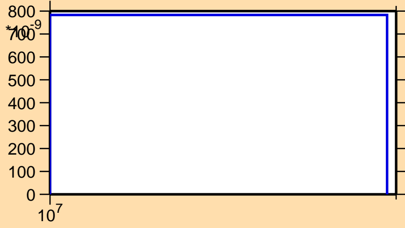
\sigma vs. E for ^{159}\text{Er}(n,2np)
