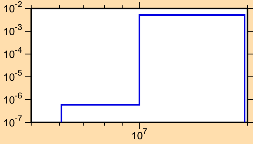
\sigma vs. E for ^{159}\text{Er}(n,np)
