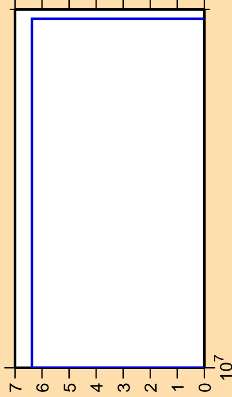
\Delta\sigma/\sigma vs. E for ^{159}\text{Er}(n,nt)
