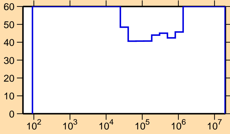
\Delta\sigma/\sigma vs. E for ^{159}\text{Er}(n,\gamma)
