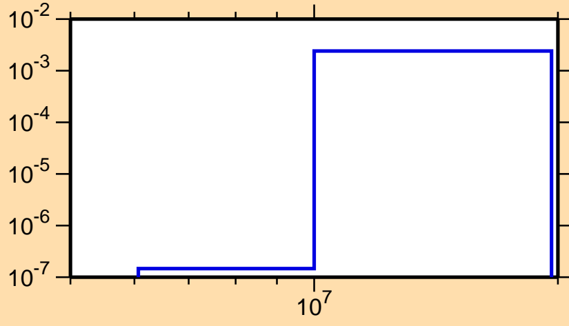
\sigma vs. E for ^{159}\text{Er}(n,d)
