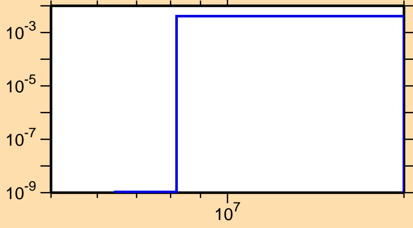
\sigma vs. E for ^{159}\text{Er}(n,np)
