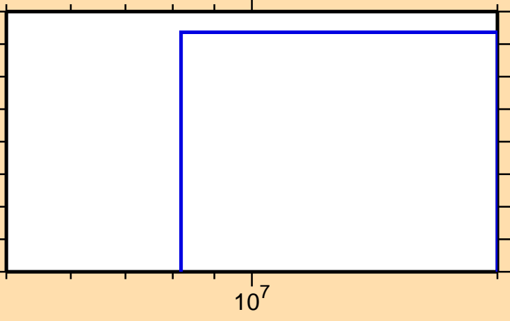
\sigma vs. E for ^{159}\text{Er}(\text{mt117})
