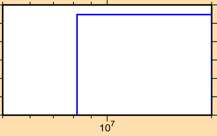
\sigma vs. E for ^{159}\text{Er}(n,3n)
