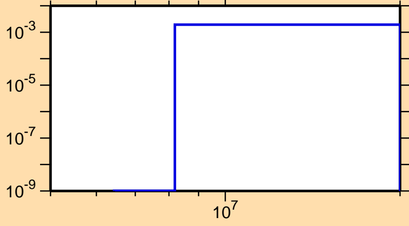
\sigma vs. E for ^{159}\text{Er}(n,d)
