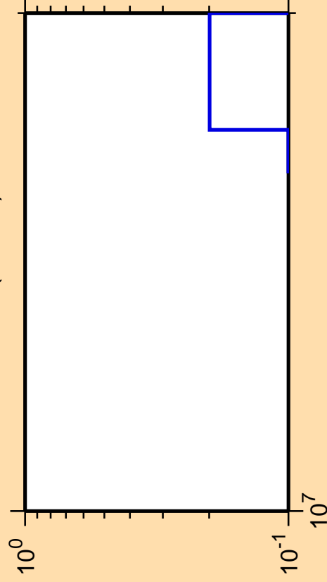
\Delta\sigma/\sigma vs. E for ^{160}\text{Er}(n,3n\alpha)
