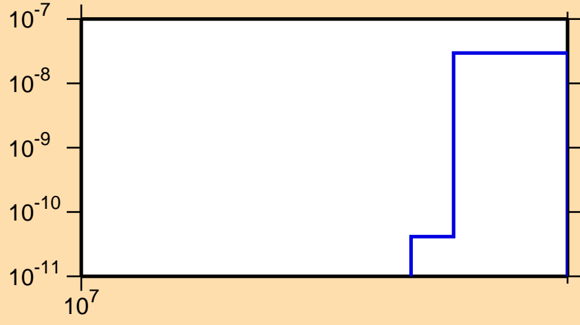
\sigma vs. E for ^{160}\text{Er}(n,\text{nd})
