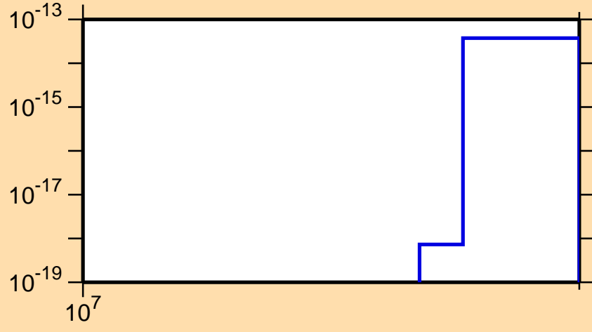
\sigma vs. E for ^{160}\text{Er}(n,3n\alpha)
