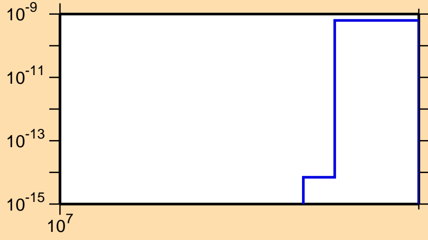
\sigma vs. E for ^{161}\text{Er}(n,nt)
