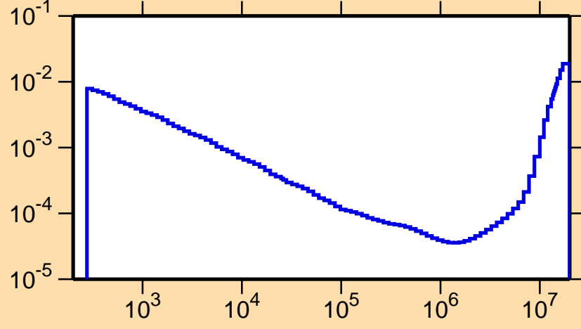
\sigma vs. E for ^{161}\text{Er}(n,\alpha)
