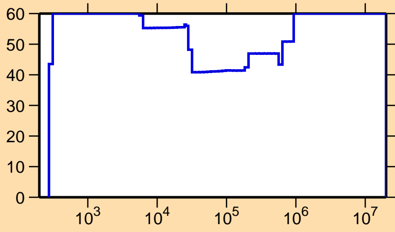
\Delta\sigma/\sigma vs. E for ^{161}\text{Er}(n,\gamma)
