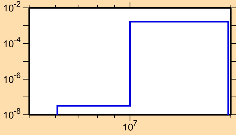
\sigma vs. E for ^{161}\text{Er}(n,d)
