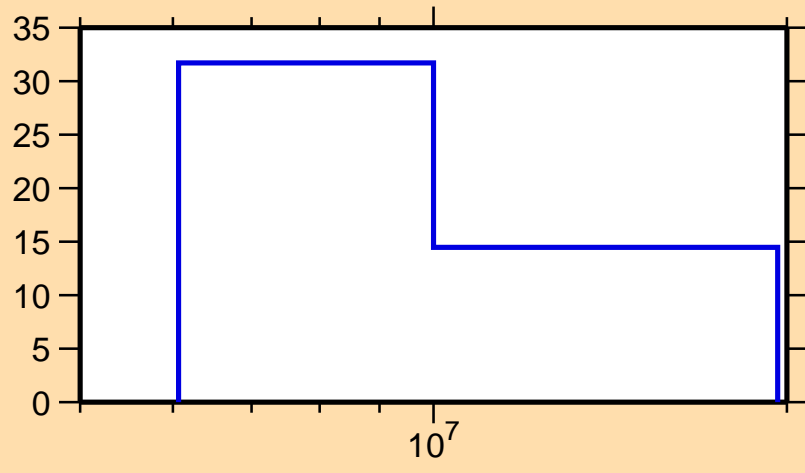
\Delta\sigma/\sigma vs. E for ^{161}\text{Er}(n,2n)
