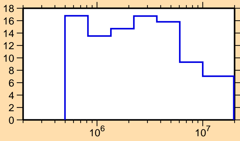
\Delta\sigma/\sigma vs. E for ^{161}\text{Er}(n, el.)
