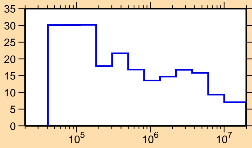
\Delta\sigma/\sigma vs. E for ^{161}\text{Er}(n,\text{el.})
