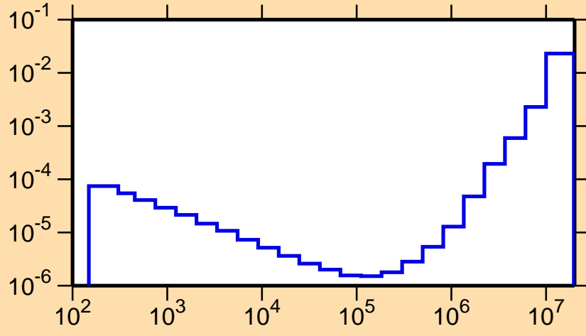
\sigma vs. E for ^{161}\text{Er}(n,p)
