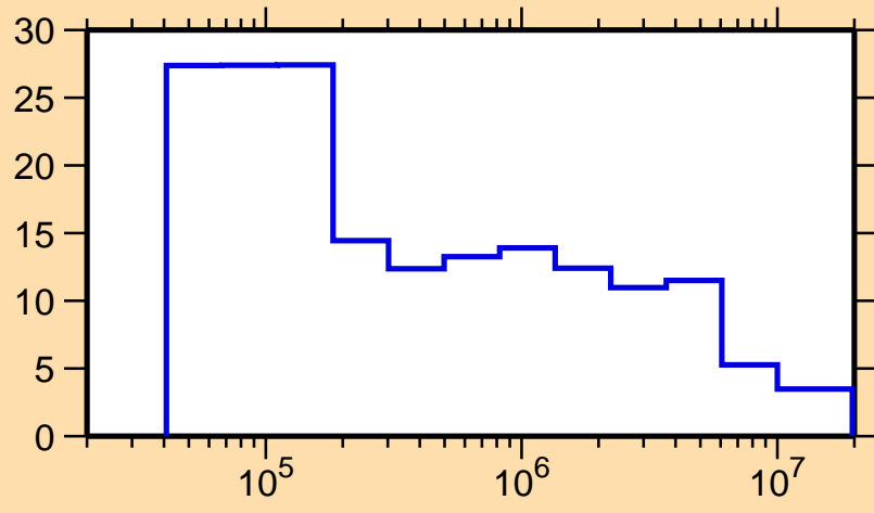
\Delta\sigma/\sigma vs. E for ^{161}\text{Er}(n,\text{tot.})
