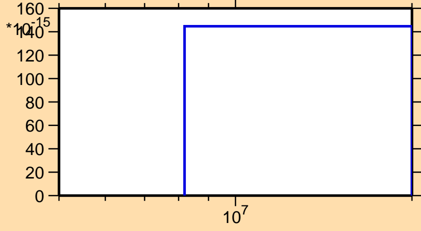
\sigma vs. E for ^{161}\text{Er}(\text{mt } 45)
