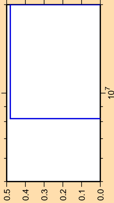
\Delta\sigma/\sigma vs. E for ^{161}\text{Er}(n,pd)
