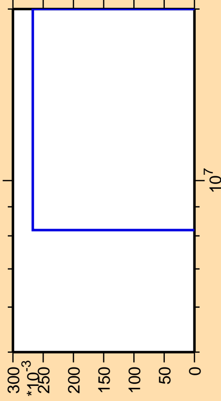
\Delta\sigma/\sigma vs. E for ^{161}\text{Er}(\text{mt } 45)
