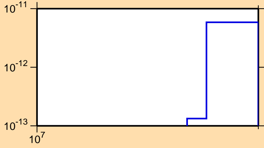
\sigma vs. E for ^{162}\text{Er} (mt 45)
