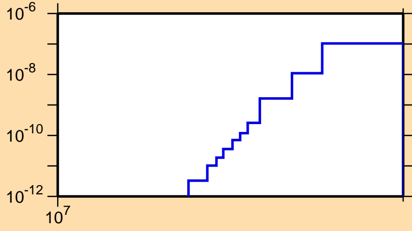
\sigma vs. E for ^{162}\text{Er}(n,\text{He3})
