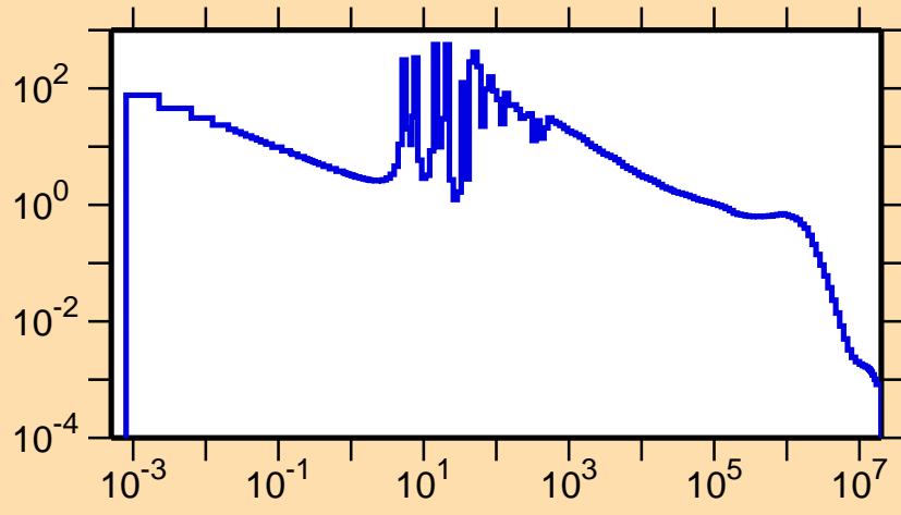
\sigma vs. E for ^{162}\text{Er}(n,\gamma)
