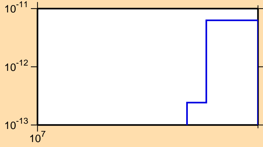
\sigma vs. E for ^{162}\text{Er}(\text{mt117})
