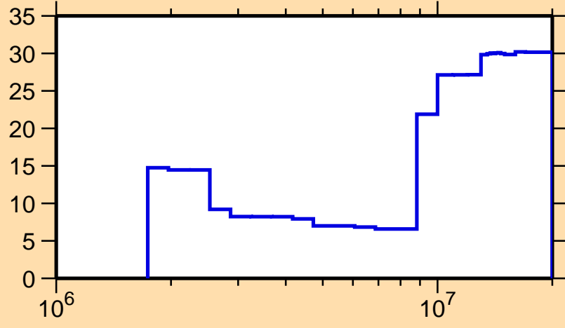
\Delta\sigma/\sigma vs. E for ^{162}\text{Er}(n,n\text{cont.})
