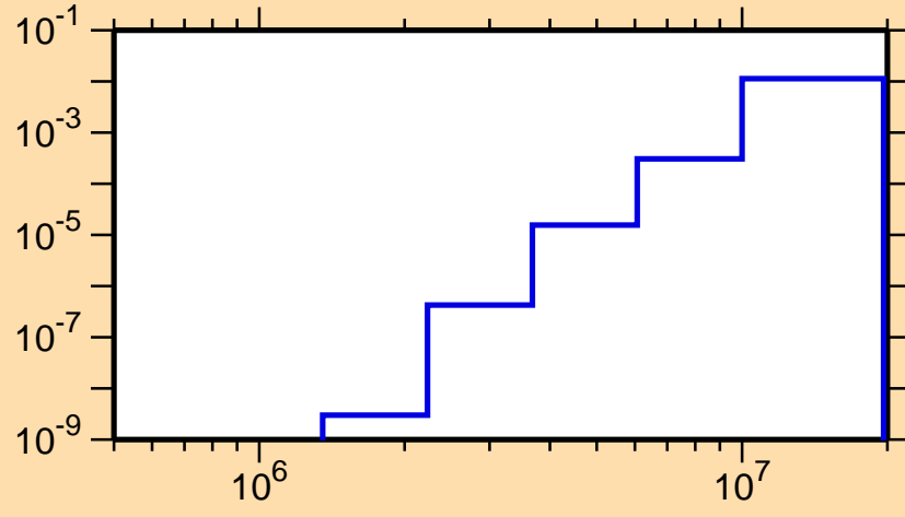
\sigma vs. E for ^{162}\text{Er}(n,p)
